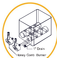
Tube-Fire Heating System for GDF12 & GDF11D
