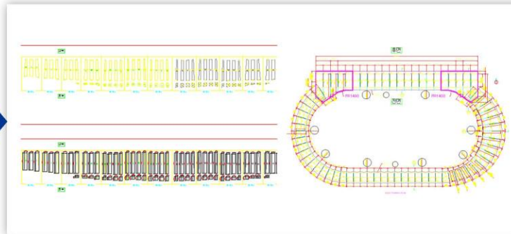
Pattern Analysis
