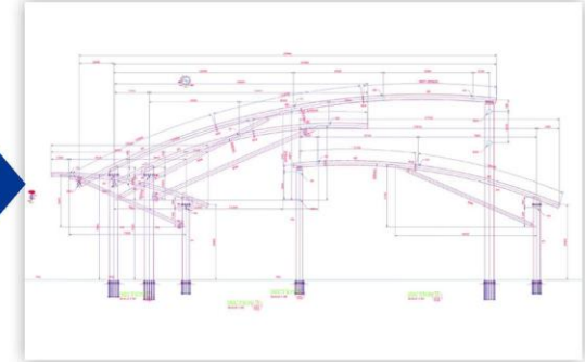
Detail Drawing
