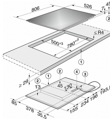
KM 6357 PowerFlex (Installation drawing) - VG AUS
