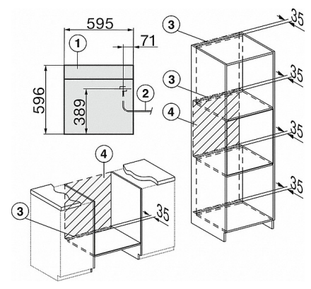
DGC7x60, DGC7x60X installation drawings
