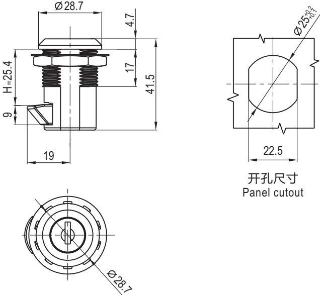
锌合金 Zinc die, bright chrome
