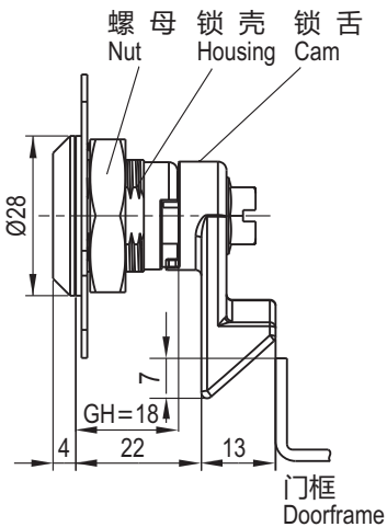
L型（左开）Version L(Left)
