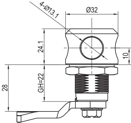
锁壳带4个挂锁孔 Housing with 4 padlock holes
