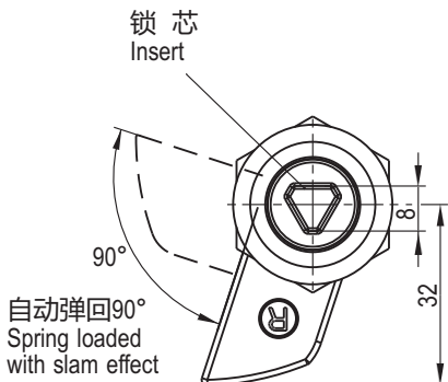
R型（右开）Version R(Right)
