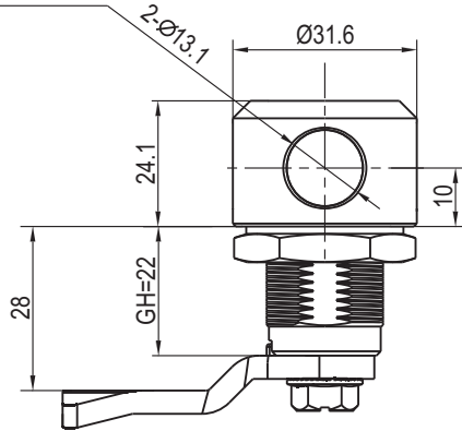
锁壳带2个挂锁孔 Housing with 2 padlock holes
