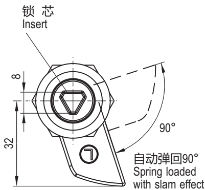
L型（左开）Version L(Left)
