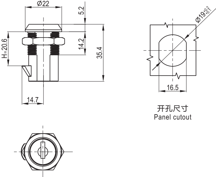
锌合金 Zinc die, bright chrome
