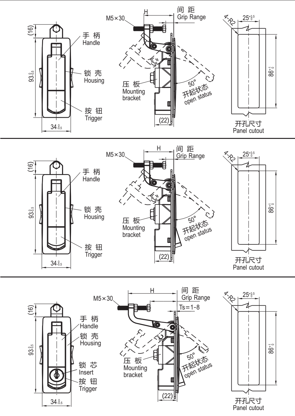
黑色锌合金基座、手柄、按钮；镀锌钢安装件 Zinc die handle ,housing and trigger black powder coated or bright chrome; m.s. zinc plated screw and fixing parts
