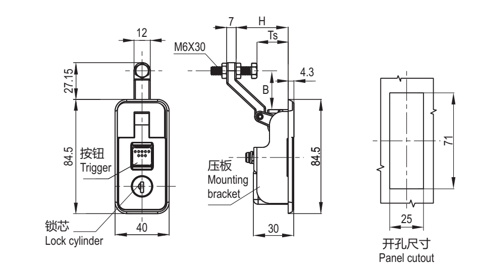
黑色锌合金基座、手柄、按钮；镀锌钢安装件 Zinc die handle, housing and trigger; m.s. zinc plated fixing parts
