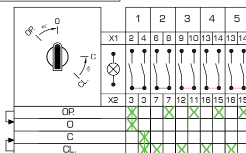
Circuit Arrangement n° DO5_08
