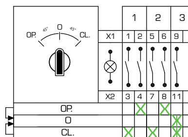
Circuit Arrangement n° SCO3_01(2-1)
