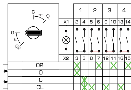
Circuit Arrangement n° D04_01
