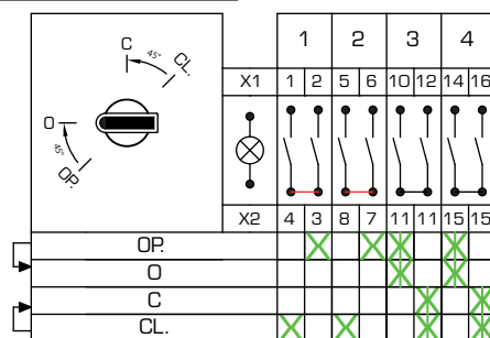
Circuit Arrangement n° D04_06(2-2)
