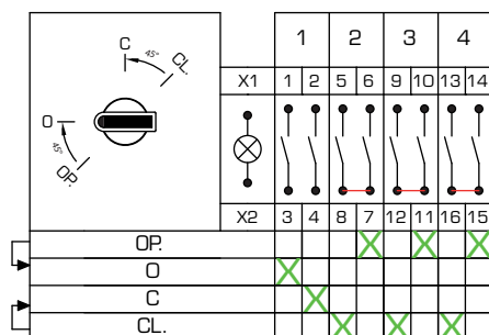
Circuit Arrangement n° DD4_43(1-3)
