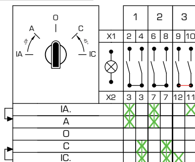
Circuit Arrangement n° F03_02
