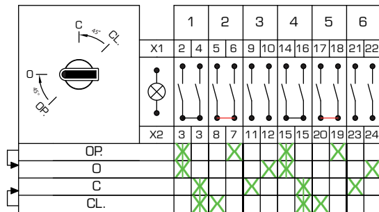
Circuit Arrangement n° E06_01
