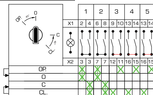
Circuit Arrangement n° DO5_15
