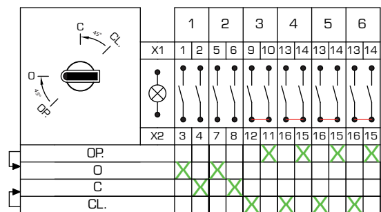
Circuit Arrangement n° D06_43(2-4)
