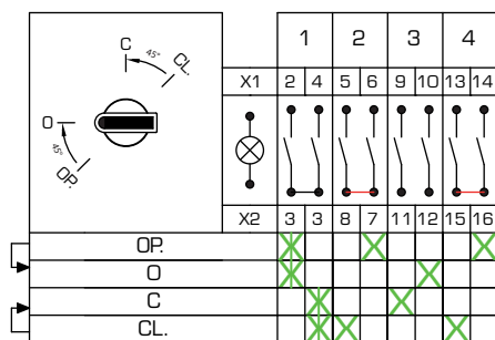
Circuit Arrangement n° E04_01
