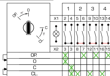
Circuit Arrangement n° D04_08
