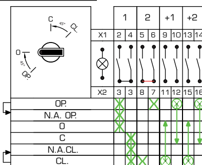
Circuit Arrangement n° T02+2_01
