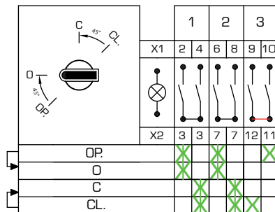
Circuit Arrangement n° D03_02
