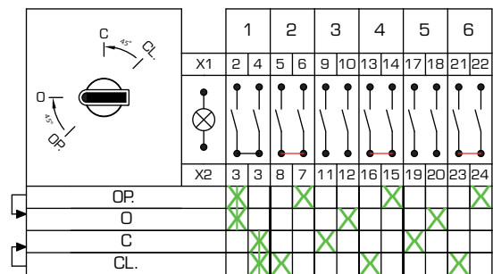
Circuit Arrangement n° E06_14(1-3)
