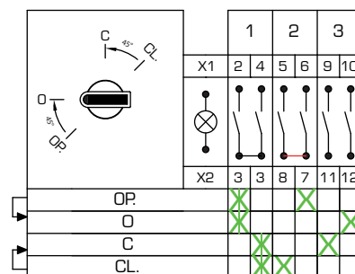
Circuit Arrangement n° E03_01
