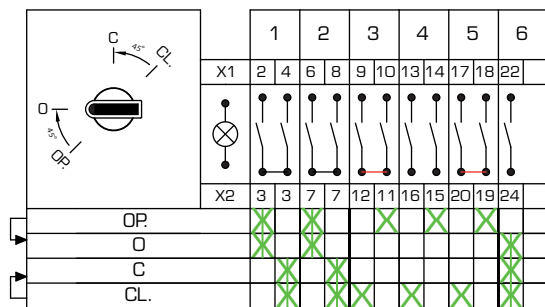
Circuit Arrangement n° D06_50(2-3-1)
