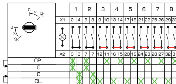
Circuit Arrangement n° D08_02
