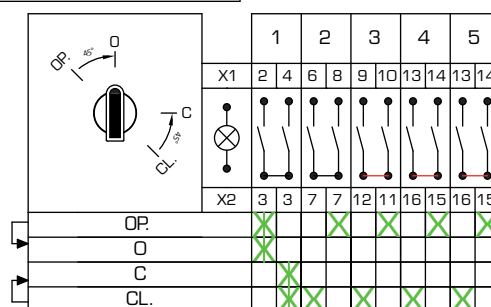
Circuit Arrangement n° DD5_08
