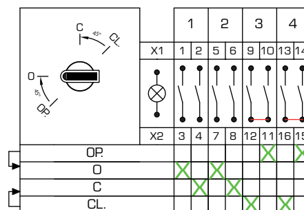
Circuit Arrangement n° DD4_43(2-2)
