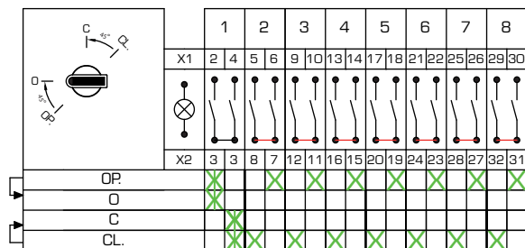
Circuit Arrangement n° D08_01
