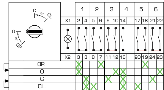
Circuit Arrangement n° E06_52(1-2)
