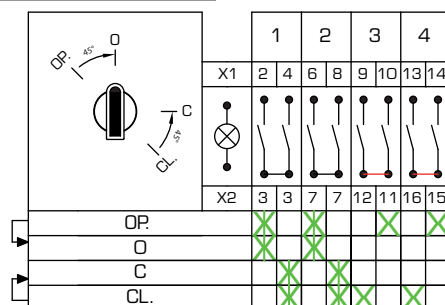
Circuit Arrangement n° D04_15
