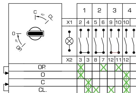
Circuit Arrangement n° D04_51(1-2-1)
