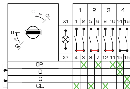
Circuit Arrangement n° D04_05
