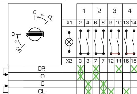
Circuit Arrangement n° D04_02
