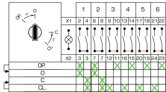
Circuit Arrangement n° D06_08
