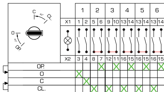
Circuit Arrangement n° D06_43(1-5)
