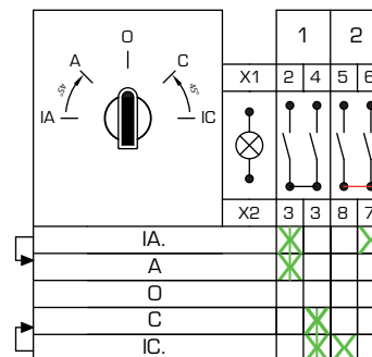
Circuit Arrangement n° F04_01
