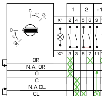
Circuit Arrangement n° T02+1_01
