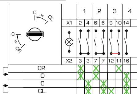
Circuit Arrangement n° DO4_50(2-1-1)
