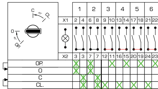
Circuit Arrangement n° D06_02
