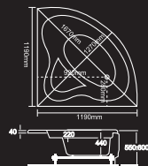
Model: 3200 - Size: 1200 x 1200 x 440 mm
