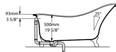
Section AA
