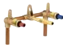
Rough-in wallmount valve MCL9700
