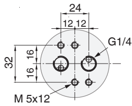
Detail X ADA/ASR 0020U-1750U
