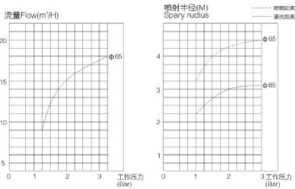
清洗球曲线图-Q65 Performance curve-Q65
