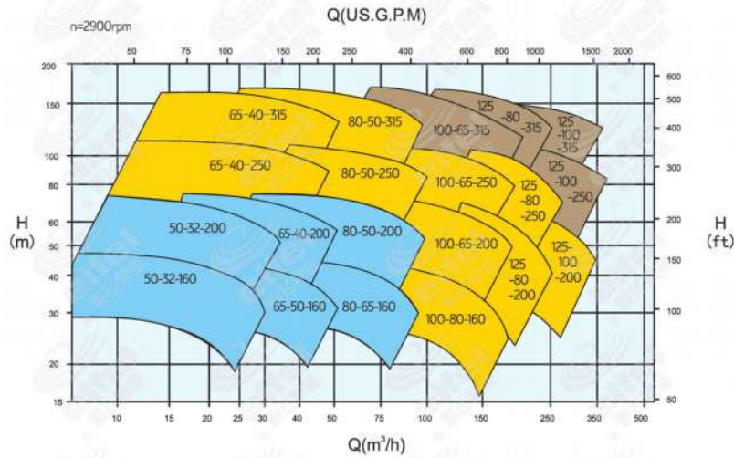
EH Series-50Hz Performance
