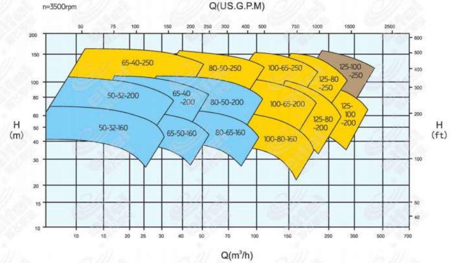
EH Series-60Hz Performance
