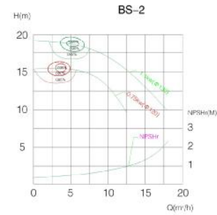
BS系列离心泵性能曲线图 BS Series pump performance curve figure
