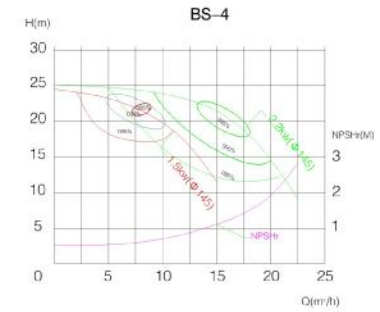
BS系列离心泵性能曲线图 BS Series pump performance curve figure
