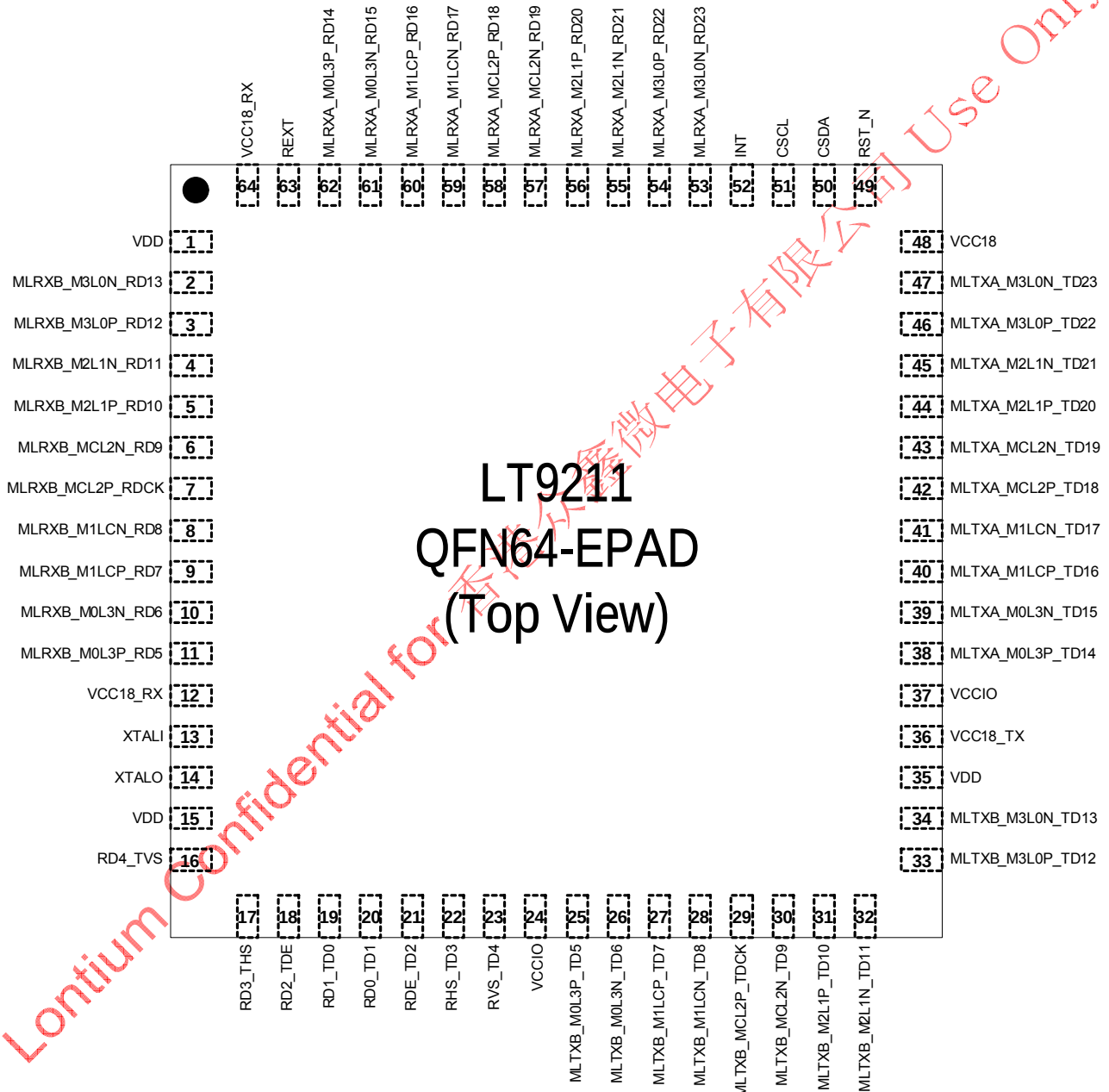
Figure 7.1.1 QFN64 Pin Configuration
