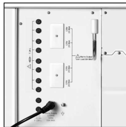
Fuse Panel
